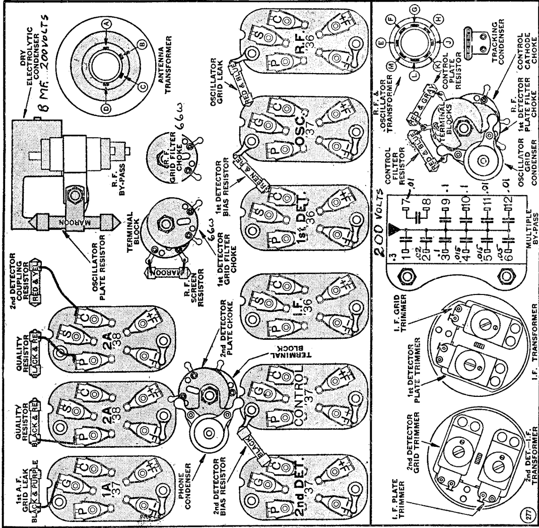
BOTTOM CHART OF MODEL 91, 91-B AND 91-C.
